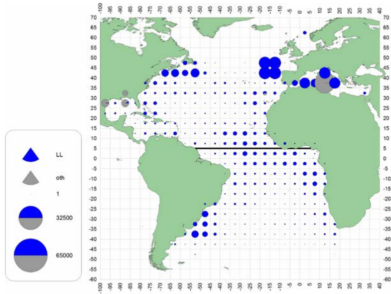
c. SWO (1970-79)
