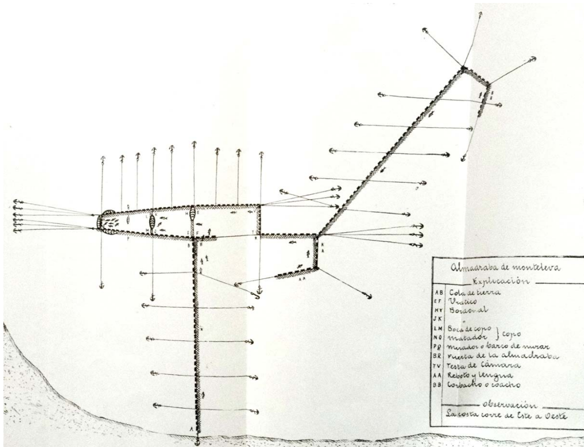
Figure 7. Traditional set-type tuna trap (almadraba de monteleva, in a particular configuration) (from Rodriguez Santamaria, 1920).
