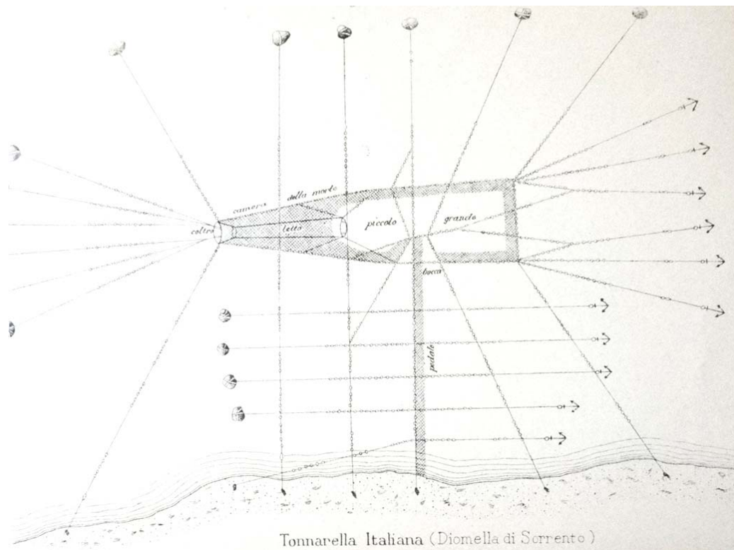
Figure 8. Traditional small set-type tuna trap ("tonnarella" or "petit madrague") (from Parona, 1919).
