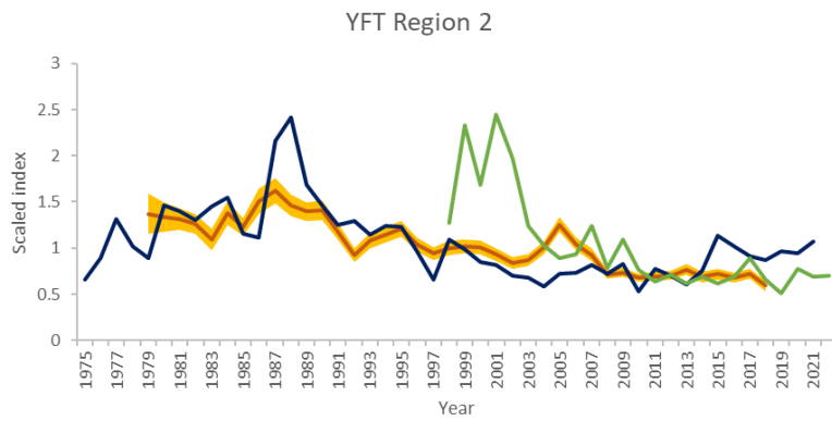
— 2019 Joint LL_R2_with95%CI — 2023 JPNLL_R2 — BRALL_R2
