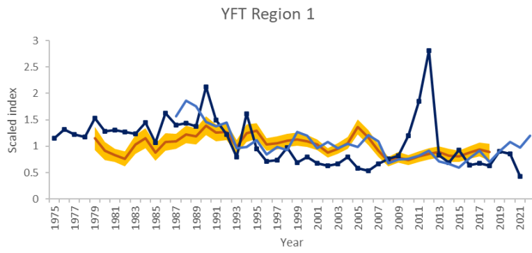
— 2019 Joint LL_R1_with95%CI — 2023 JPNLL_R1 — 2023_USLL
