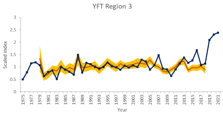
— 2019 Joint LL_R3_with95%CI — 2023 JPNLL_R3
