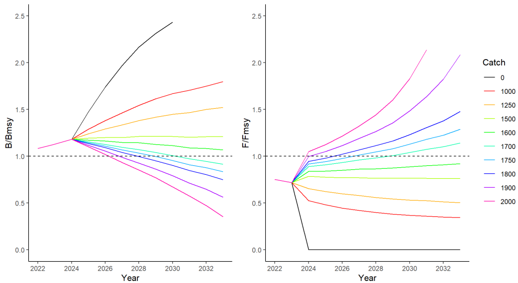
SAI-Figure 10. Projections for B/B_{MSY} and F/F_{MSY} for the West Atlantic sailfish stock for various levels of future constant catch ranging from 1,000 – 2,000 t, including a zero-catch scenario starting in 2024. The initial catch for the years 2022-2023 was set to 1,313 t, which is the geometric mean catch of the recent three years (2019-2021). The projections were run until 2033 (10 years).
