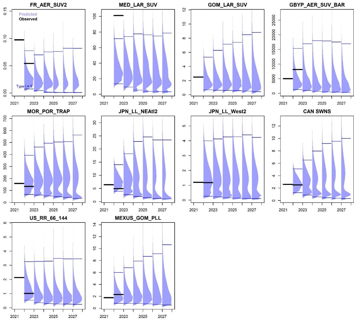
Figure 19.18.2. Plots of observed individual indices (black bars) and distribution of predicted data (blue density distribution) for the reference grid of operating models ( n = 2304 , 48 operating models, 48 simulations each). Blue bars represent the 95% intervals.
