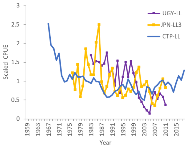
ALB-AT-Figure 5. South Atlantic albacore. Standardized catch rates used for the base case of the 2020 Stock Assessment (Anon. 2020j).
