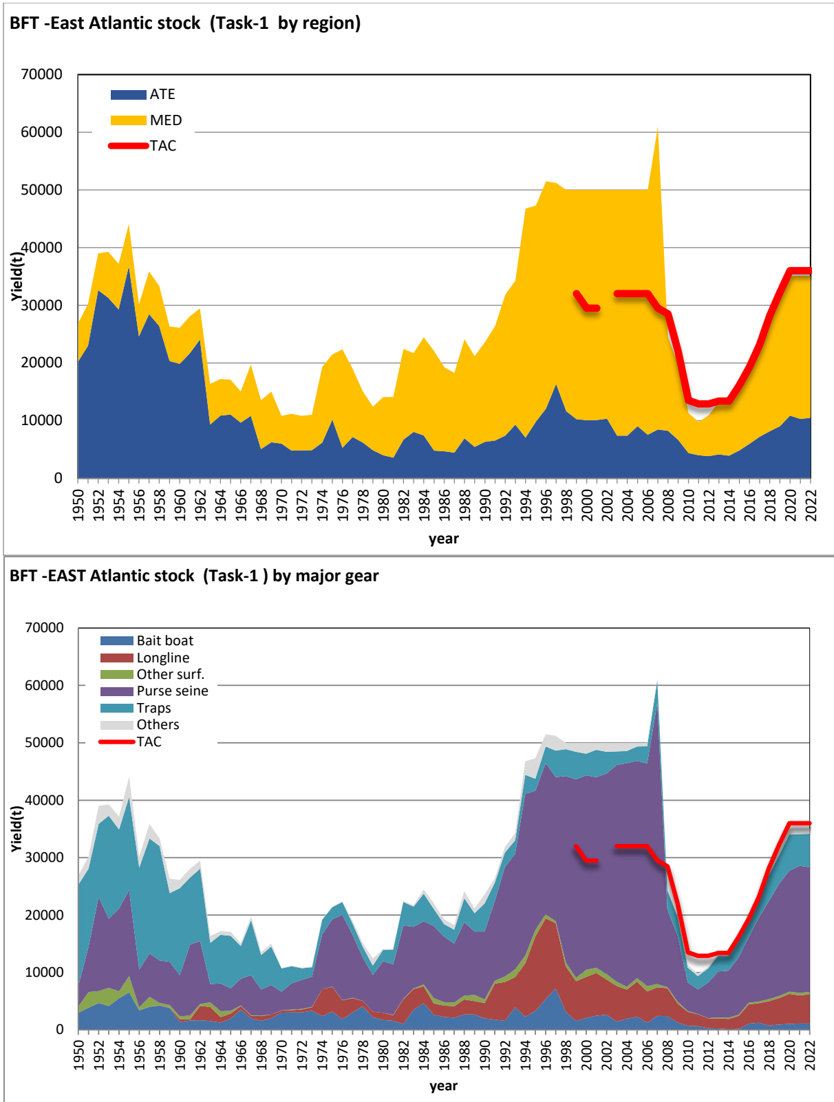
BFTE-Figure 1. Reported catch for the East Atlantic and Mediterranean from Task 1 data from 1950 to 2022 split by main geographic areas (top panel) and by gears (bottom panel) together with unreported catch estimated by the Committee from 1998 to 2007 and TAC levels since 1998.
