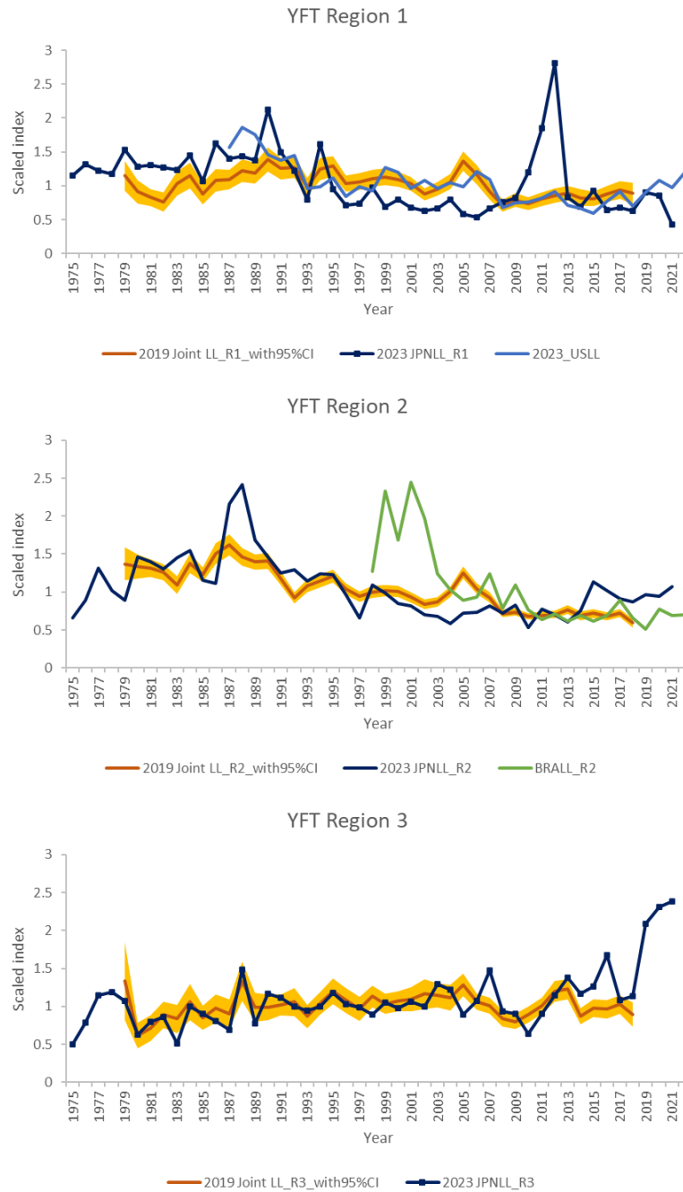
YFT-Figure 8. Comparisons of abundance indices updated in 2023, and the joint longline index used in the 2019 stock assessment of Atlantic yellowfin tuna, by region. The Brazilian longline index includes information for both regions 2 and 3.
