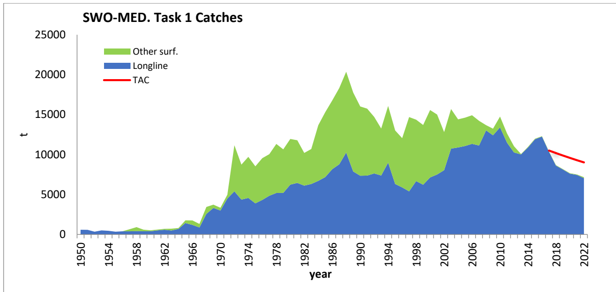
SWO-MD-Figure 1. Estimates of Task I swordfish catches (t) in the Mediterranean by major gear types, for the period 1950-2022, and corresponding annual TACs since 2017 [Rec.16-05].
