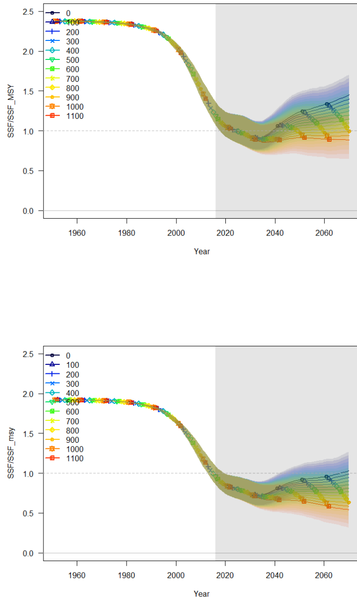
SMA-Figure 8. Constant catch projections (0 – 1100 t) from Stock Synthesis model run 1 (top panel) and run 3 (bottom panel) for the North Atlantic shortfin mako (Anon. 2019g). Solid lines are medians and shaded areas are 95% credible intervals.
