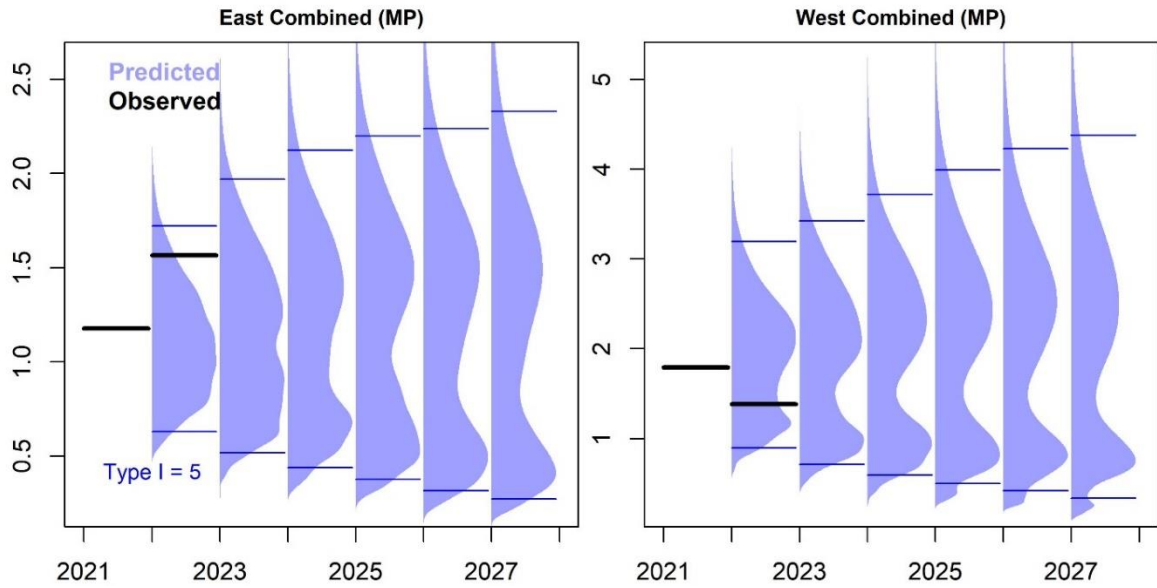
Figure 19.17.1. Standard marginal plots of observed composite indices (black bars) and distribution of predicted data (blue density distribution) for the reference grid of operating models (n =2304, 48 operating models, 48 simulations each). Blue bars represent the 95% prediction intervals.
