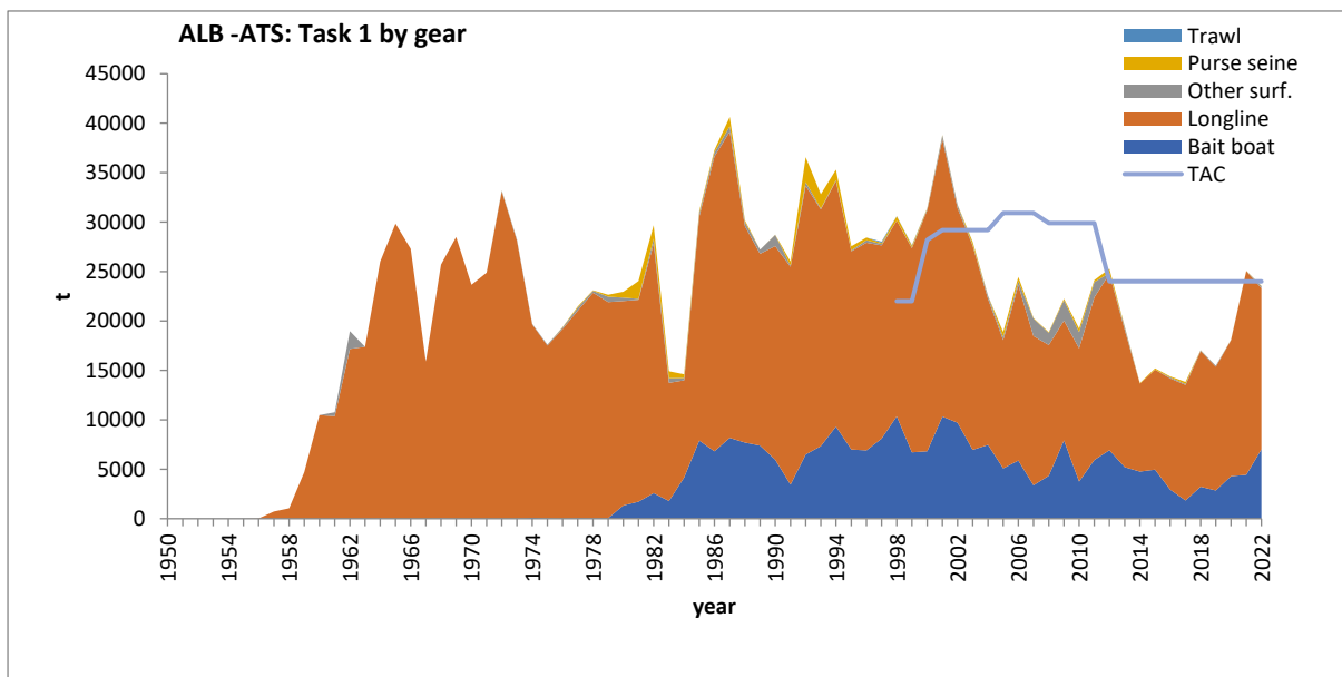
ALB-AT-Figure 2. Total albacore catches reported to ICCAT (Task I) by gear for the northern (top) and southern (bottom) Atlantic stocks including TAC.
