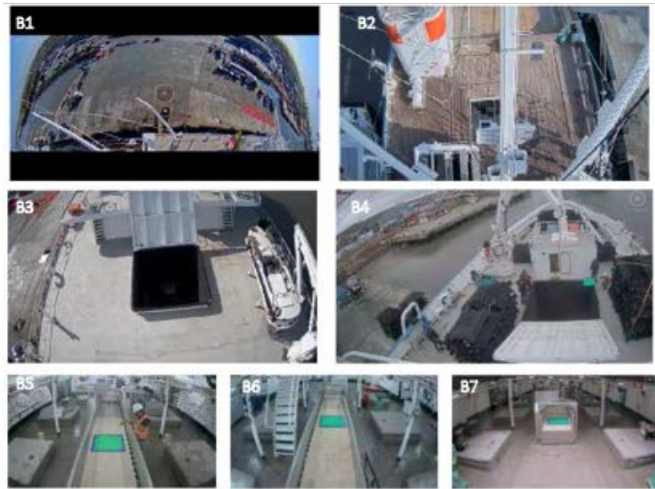
Figure 1. An example of a 7-camera EMS (four in the upper deck and three in the well deck) installed in a purse seiner covering main areas of fishing and fishing handling operations including 1 more camera in the conveyor belt: (B1) 360° Panoramic view camera (e.g port side view), (B2) Crows nest stern view camera, (B3) Working deck crane view camera, (B4) Foredeck view camera, (B5) Conveyor belt stern view camera, (B6) Conveyor belt middle camera, and (B7) Conveyor belt bow camera (source: Digital Observer Services).
