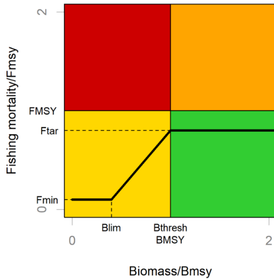
ALB-AT-Figure 7. Graphic form of the HCR adopted in Rec 17-04. B_{LIM} (set at 0.4B_{MSY} ) is the limit biomass reference point, B_{THRESH} (set at B_{MSY} ) is the point below which fishing mortality decreases linearly, F_{TAR} (set at 0.8F_{MSY} ) is the target fishing mortality rate to be applied to achieve the management objectives, and F_{MIN} (set at 0.1F_{MSY} ) is the fishing mortality to be applied when B < B_{LIM} .
