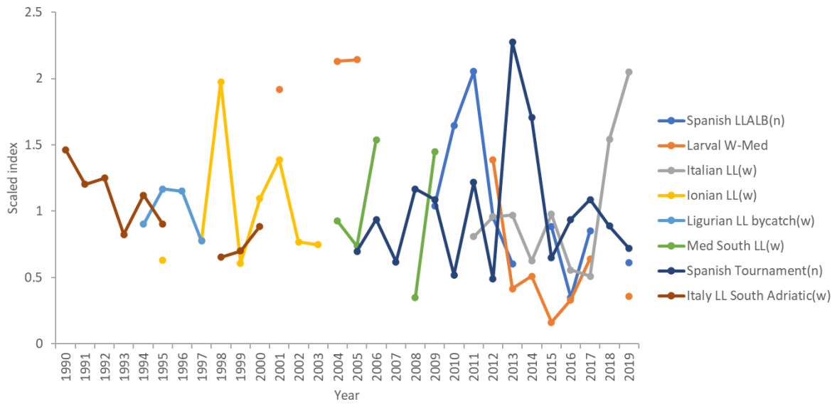
ALB-MD-Figure 3. Mediterranean albacore. Abundance indices used in the 2021 Assessment of the Mediterranean albacore stock (Anon., 2021m). n and w refer to abundance indices in number and weight, respectively.
