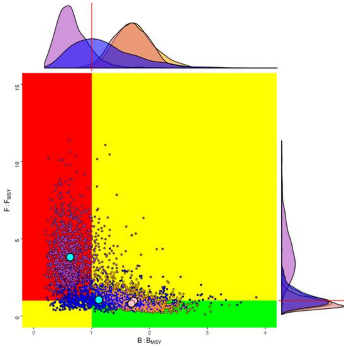
SMA-Figure 6. Stock status (2015) of South Atlantic shortfin makos based on a Bayesian production model (BSP2JAGS) and a catch-only model (CMSY). The clouds of points are the bootstrap estimates for all models combined showing uncertainty around the median point estimate for each of four model formulations (BSP2JAGS: solid pink circles; CMSY: solid cyan circles). The marginal density plots shown are the frequency distributions of the bootstrap estimates for each model with respect to relative biomass (top) and relative fishing mortality (right). The red lines are the benchmark levels (ratios equal to 1).
