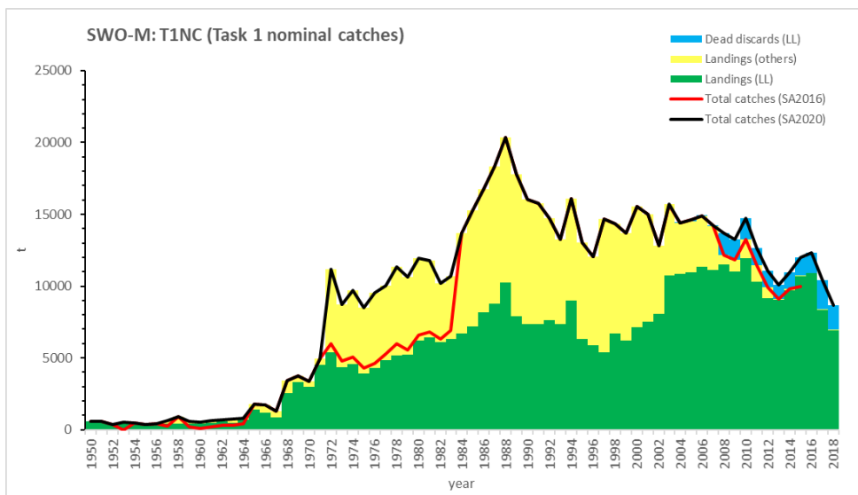
SWO-MD-Figure 2. SWO-M total nominal catches (T1NC, t) by year, showing total landings (LL and other gears) and dead discards (reported and estimated in Ortiz 2020) as prepared for the 2020 assessment. The total catches used in the 2016 stocks assessment (Anon. 2017e) is shown for comparative purposes.
