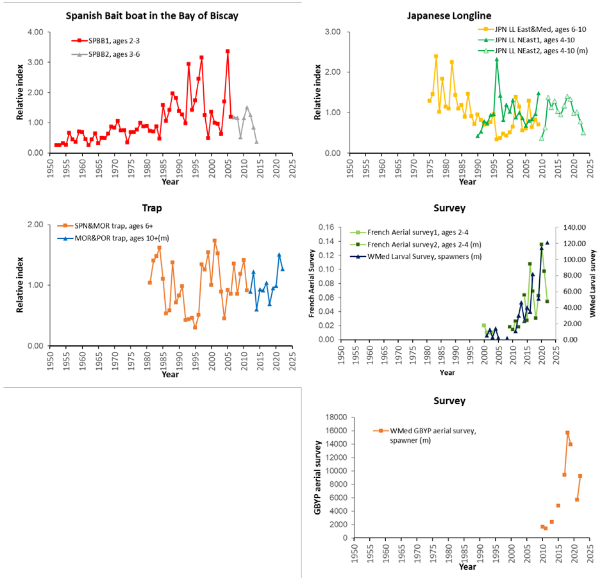
BFTE-Figure 2. Plots of the updated fishery dependent and independent indicators used for the East Atlantic and Mediterranean bluefin tuna stock. All fishery dependent indicators are standardized series and scaled to their averages. Indices denoted with a ‘m’ are used in the management procedure. The Spanish BB series was split in two series to account for changes in selectivity patterns, and the latest series was calculated using French BB data due to the sale of the quota by the Spanish fleet. The Japanese longline CPUE for the northeast Atlantic was split in 2009/2010 and the French aerial survey index was split in 2008/2009.
