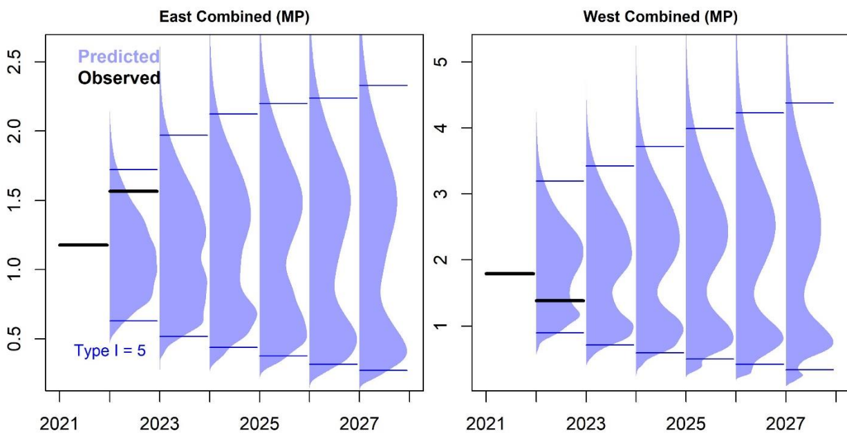
Figure 19.18.1. Standard marginal plots of observed composite indices (black bars) and distribution of predicted data (blue density distribution) for the reference grid of operating models ( n=2304 , 48 operating models, 48 simulations each). Blue bars represent the 95% intervals.
