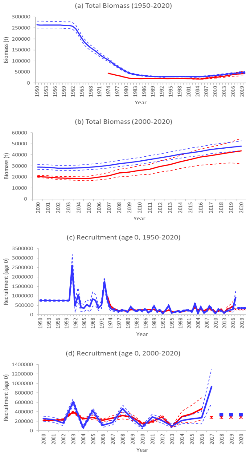
BFTW-Figure 3. Estimates of (a) total stock biomass for 1950-2020 and (b) for 2000-2020, and (c) recruitment (age 0) for 1950-2020 and (d) for 2000-2020 for the base VPA (red) and Stock Synthesis (blue) models from the 2021 assessment. The 80% confidence intervals are indicated with dashed lines. Recruitment estimates for the recent years (2017-2020 for VPA; 2018-2020 for Stock Synthesis) have been replaced by the average recruitment in the recent 6 years (2012-2017).
